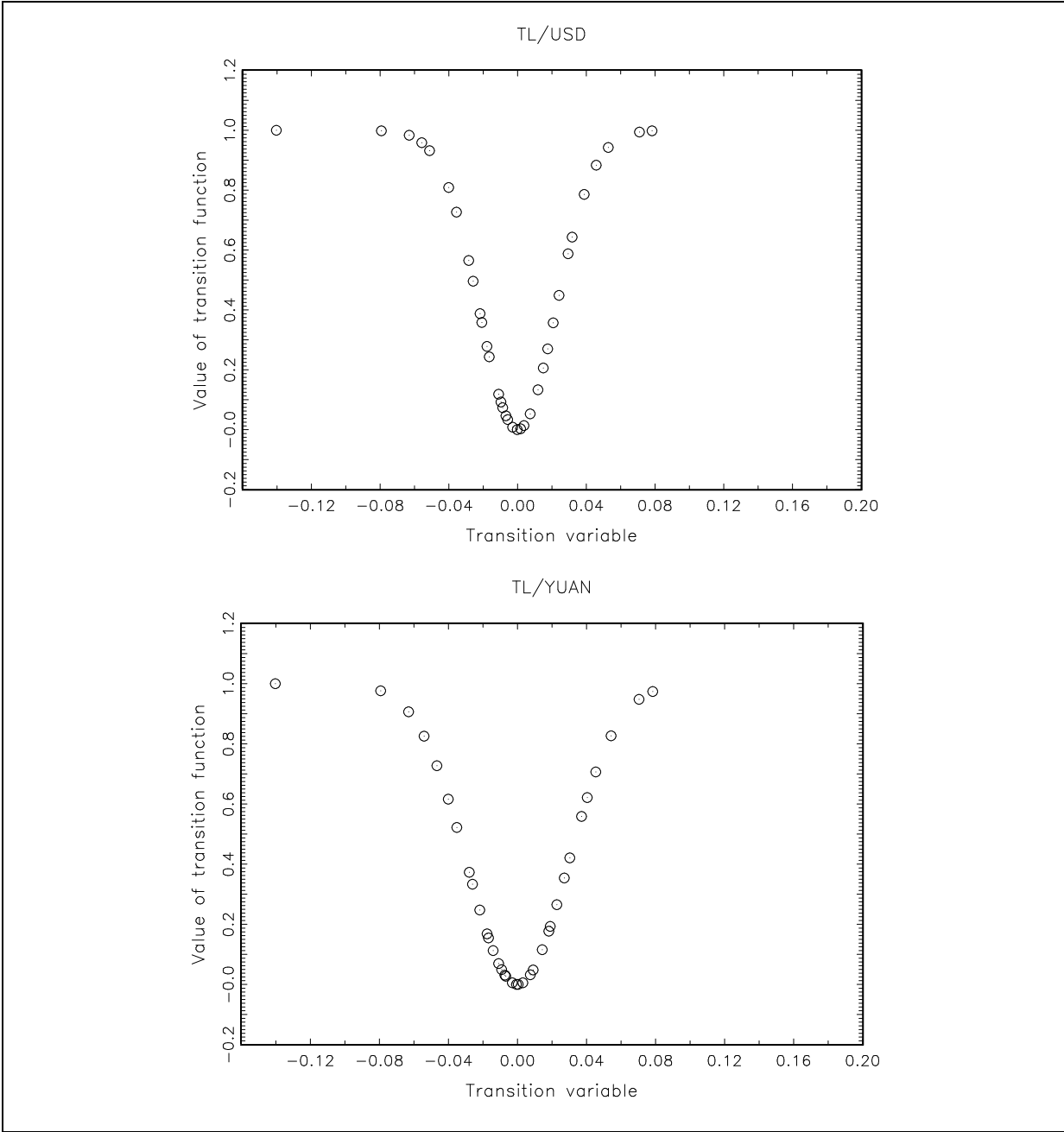
Figure 1: Scatter Plots of Estimated Transition Functions
